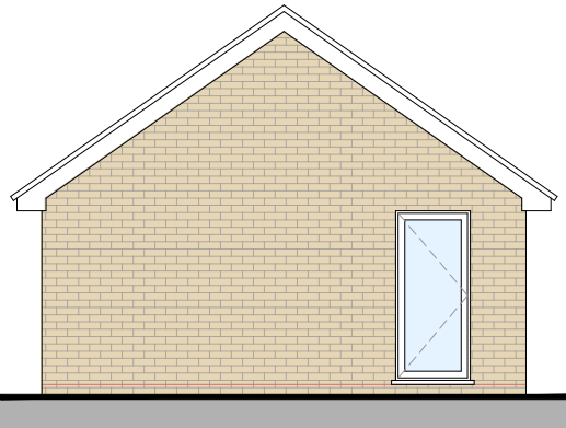
PROPOSED SOUTH ELEVATION Scale 1/100
