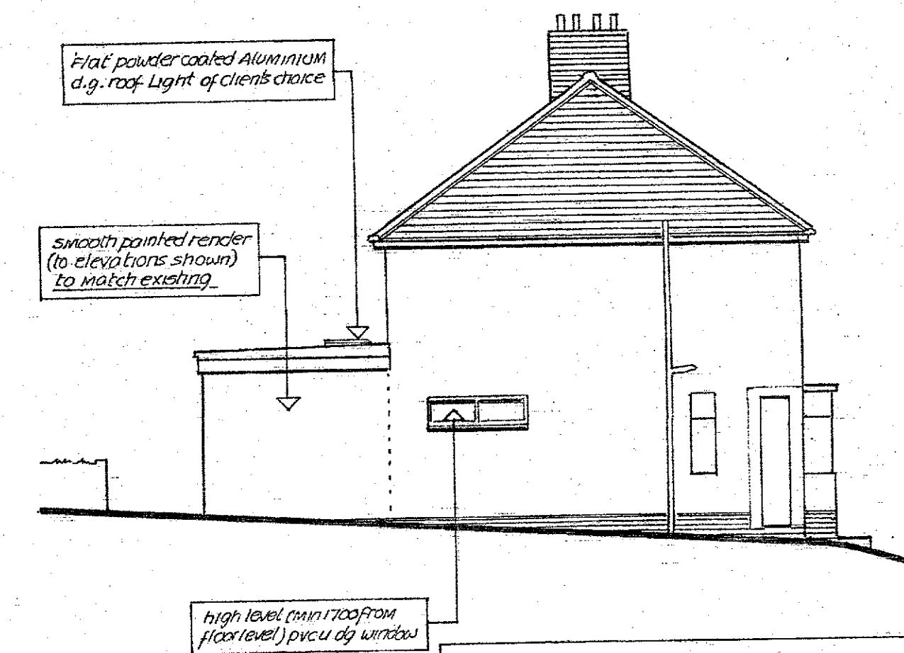
SIDE VIEW from B
