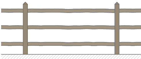
Type B 1.2m high cleft timber post and rail fence
