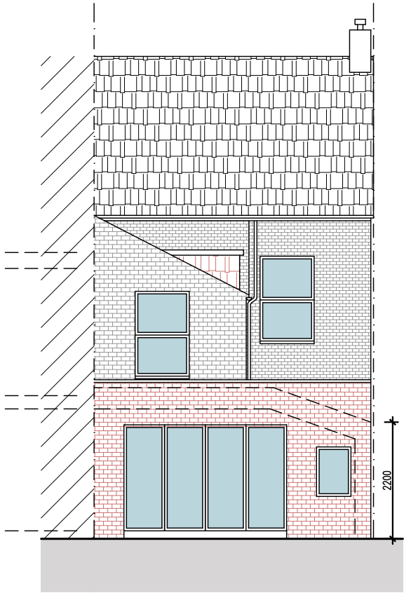
REAR ELEVATION
