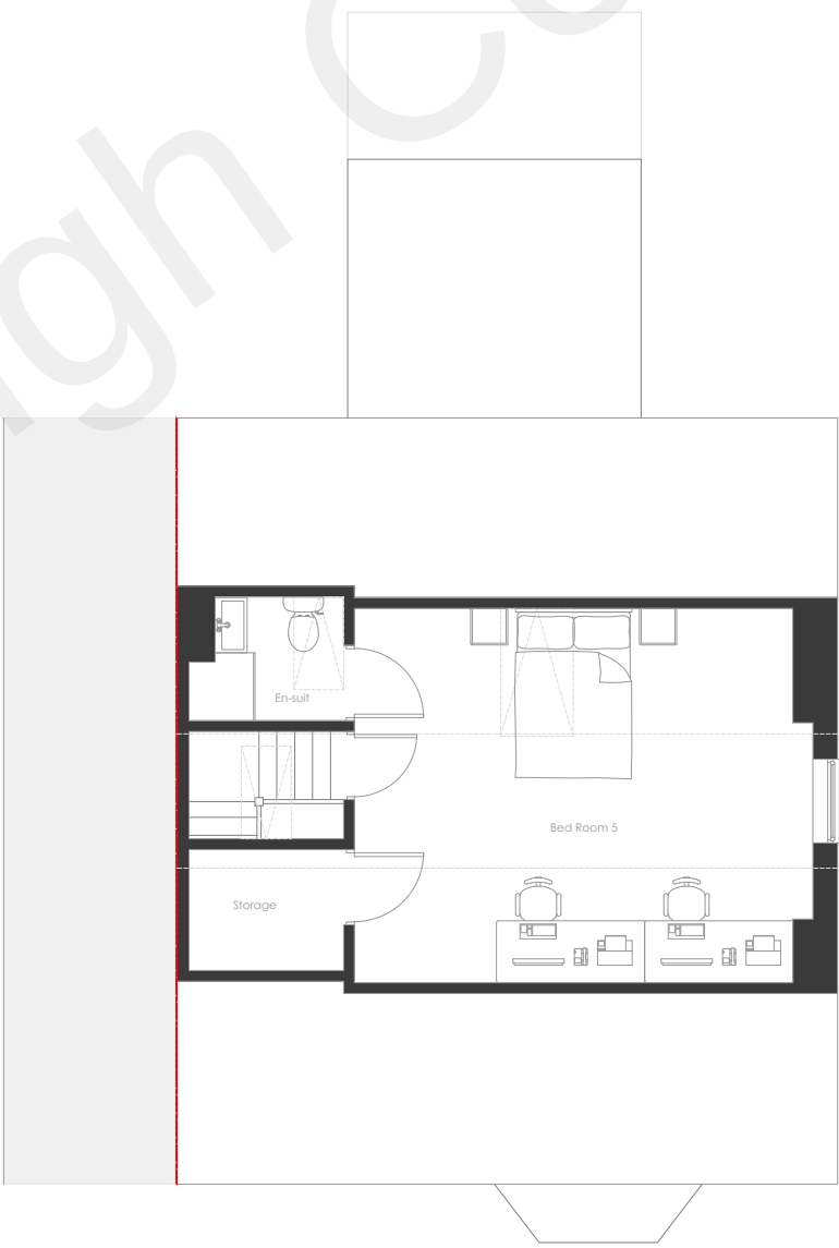
Loft Floor Plan
