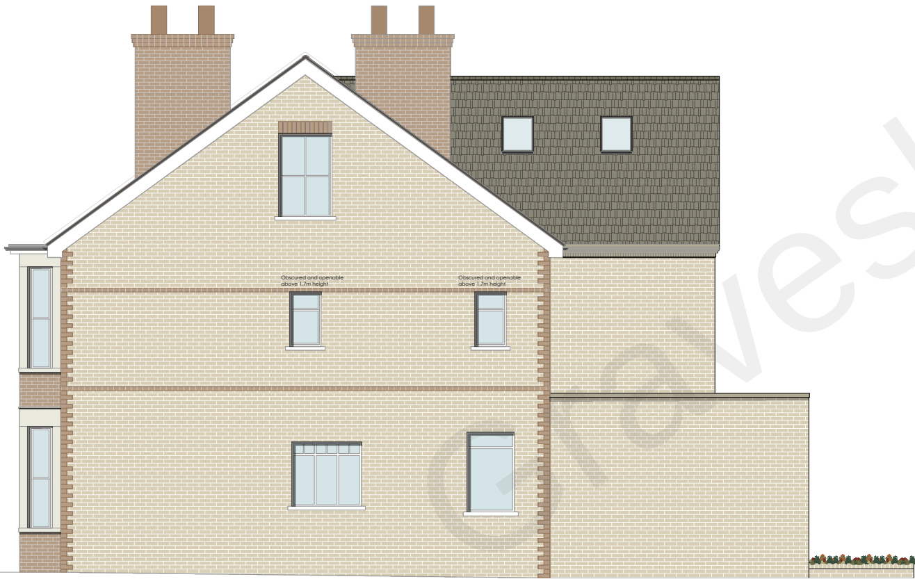
North Elevations
