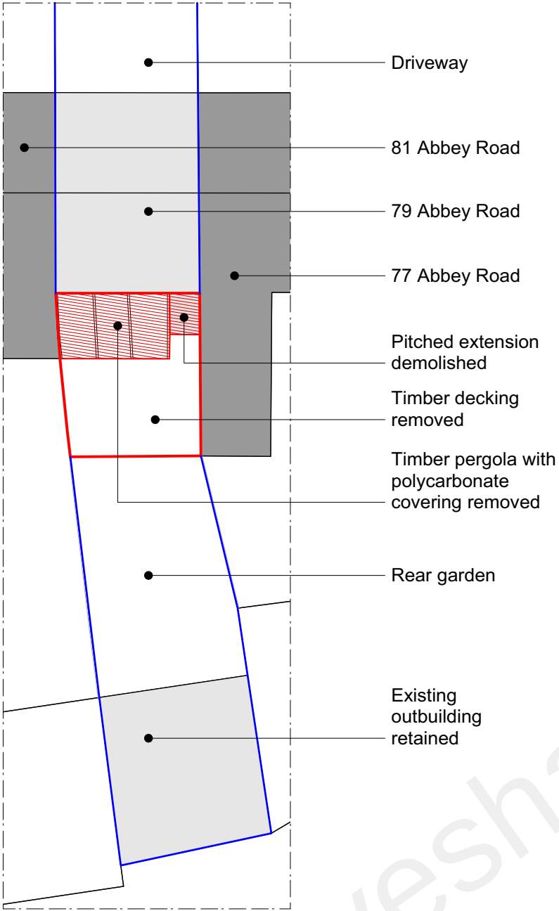
Existing block plan
