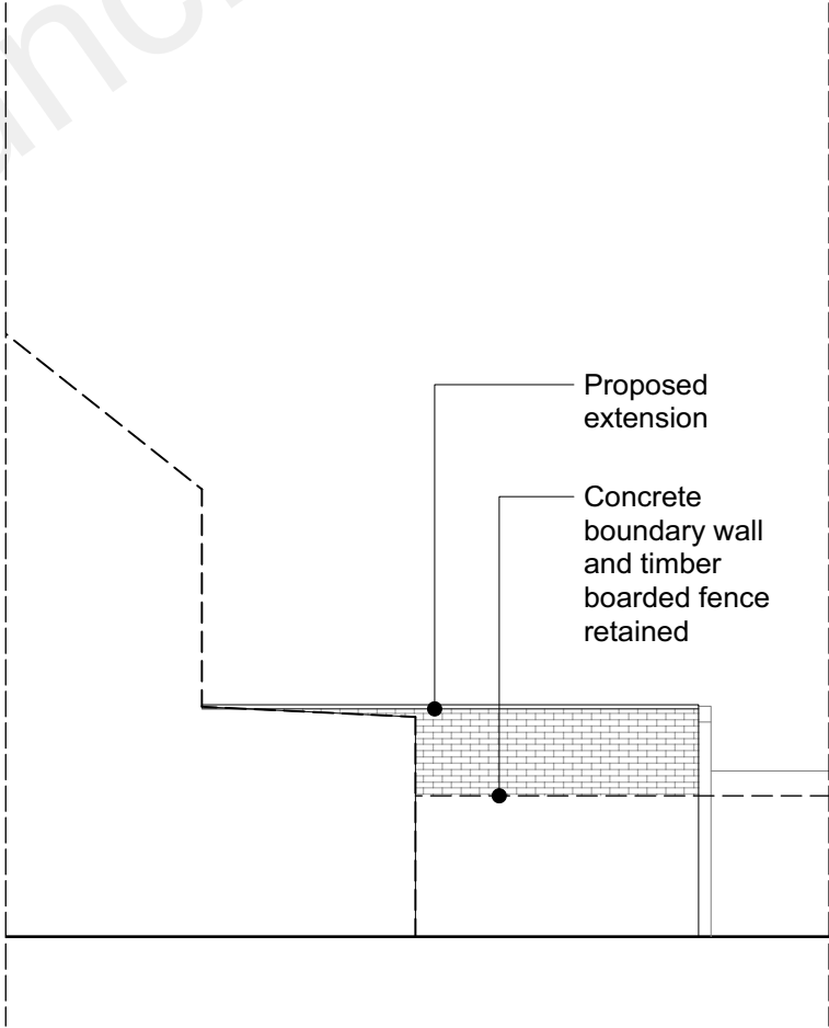
Proposed side elevation (from no. 81 Abbey Road)
