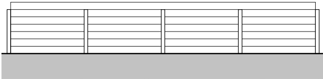
Proposed Fence Elevation (remain as existing) 1:100
