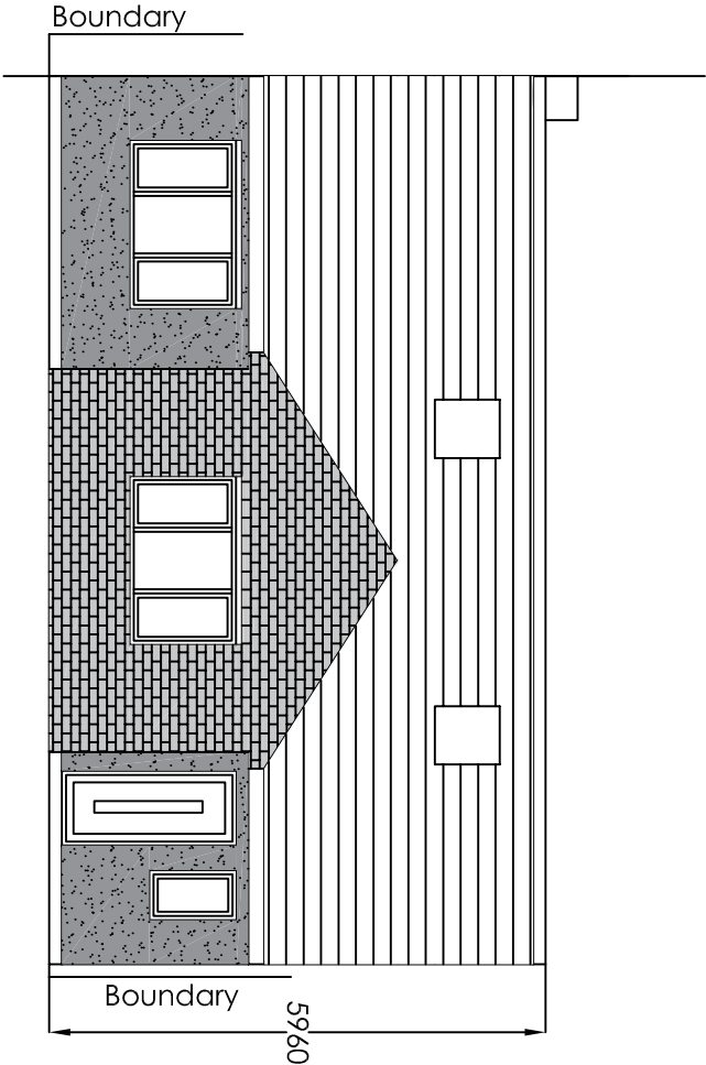
FRONT ELEVATION
