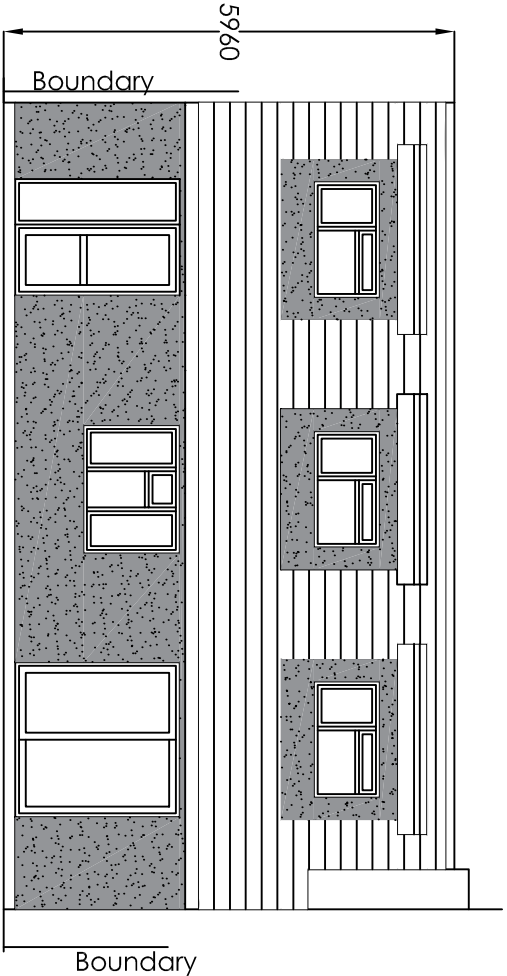
REAR ELEVATION
