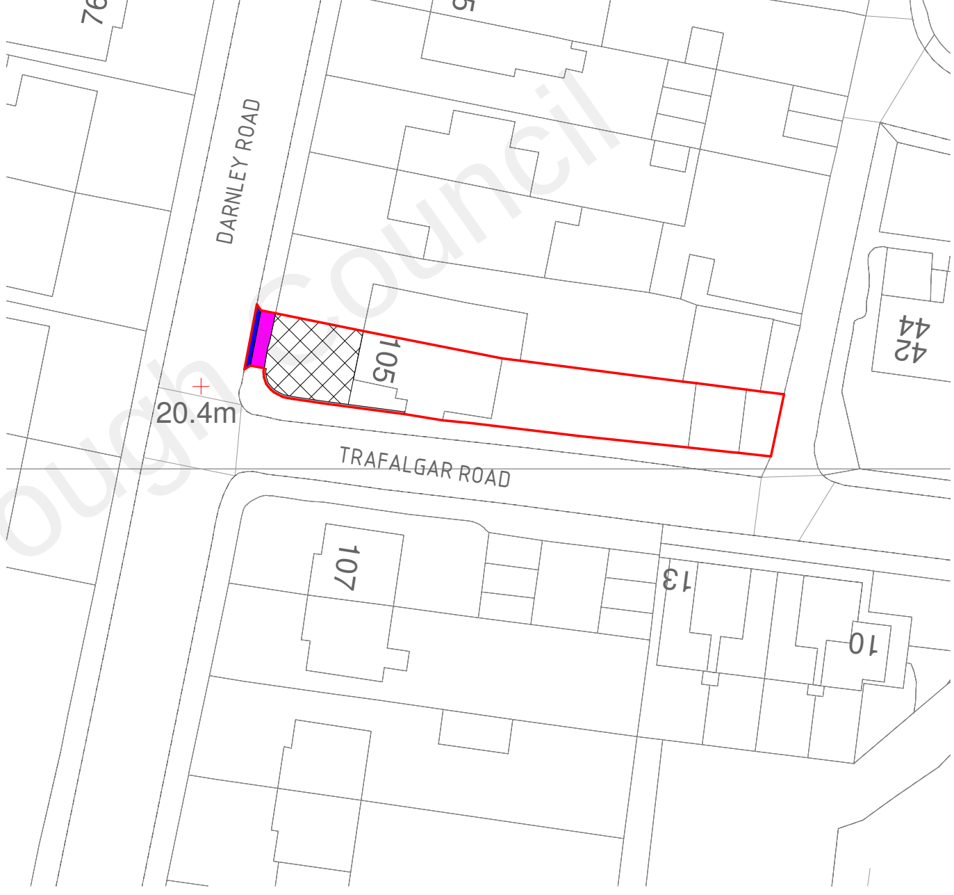
02/PBP - PROPOSED BLOCK PLAN 1: 500
