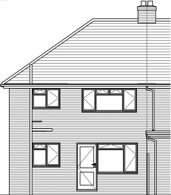
4 Rear Elevation Scale 1/100
