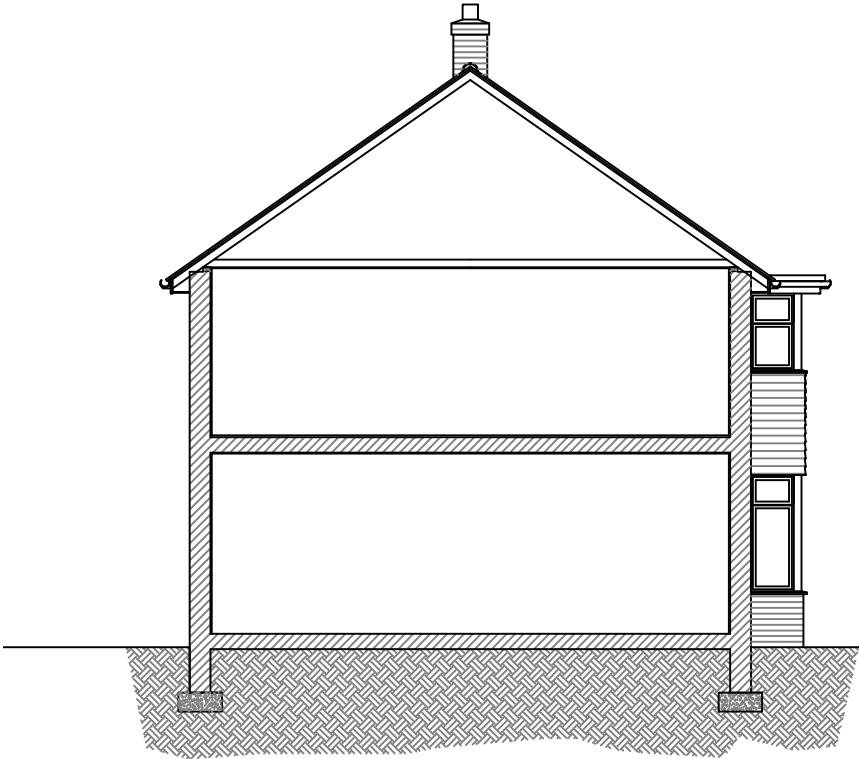
1 Sectional Elevation Scale 1/100
