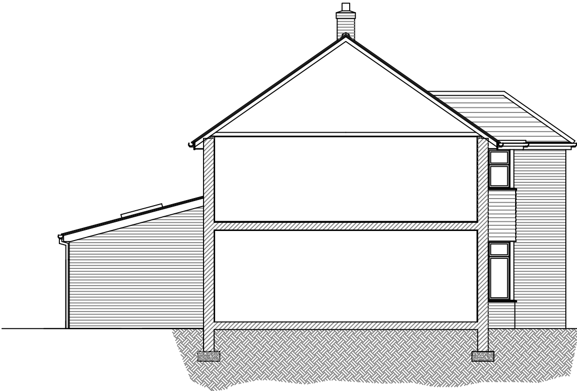
1 Sectional Elevation Scale 1/100
