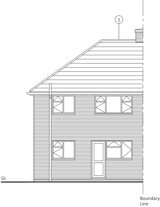
REAR (EAST) ELEVATION
