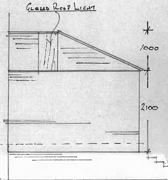
PROPOSED SOUTH ELEVATION
