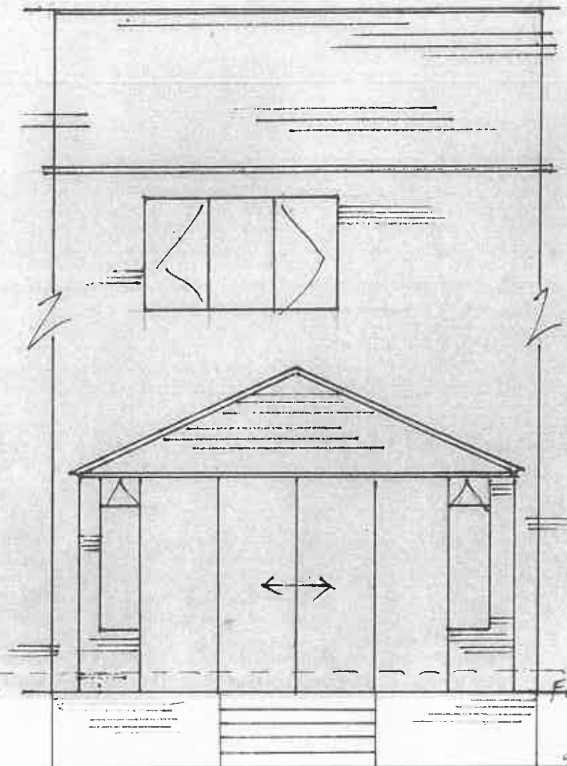
PROPOSED REAR EAST ELEVATION
