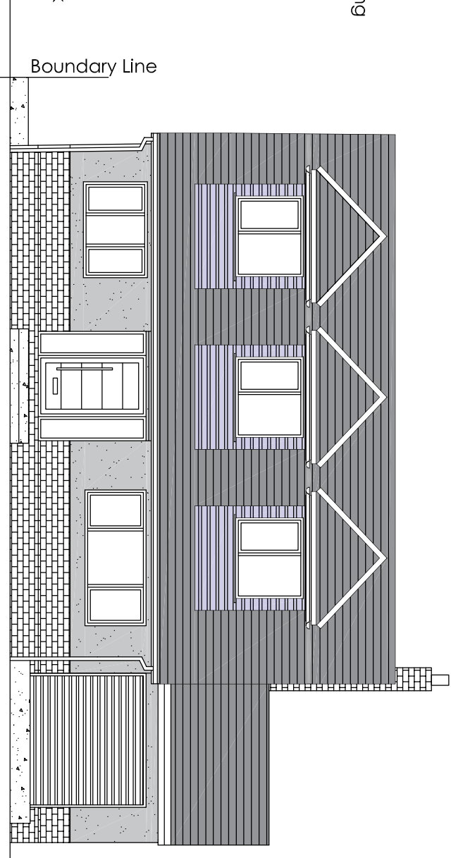
FRONT ELEVATION
