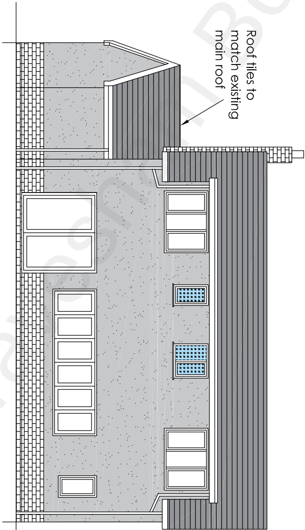
REAR ELEVATION
