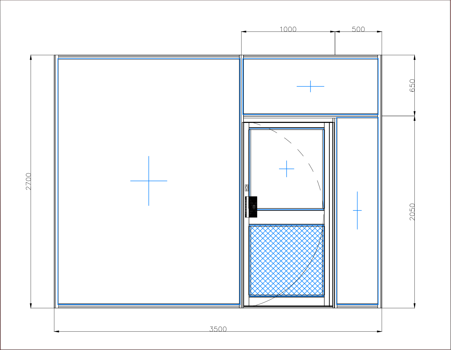
<<<<FULL WIDTH CUT THROUGH – CUT B>>>>
