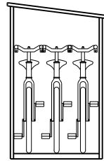
3 Bike Locker - Side 1:50
