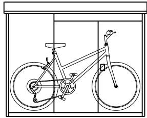
3 Bike Locker - Front 1:50
