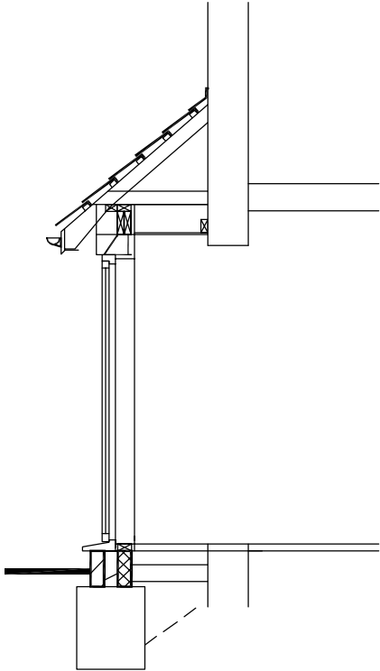
Typical Section BB
