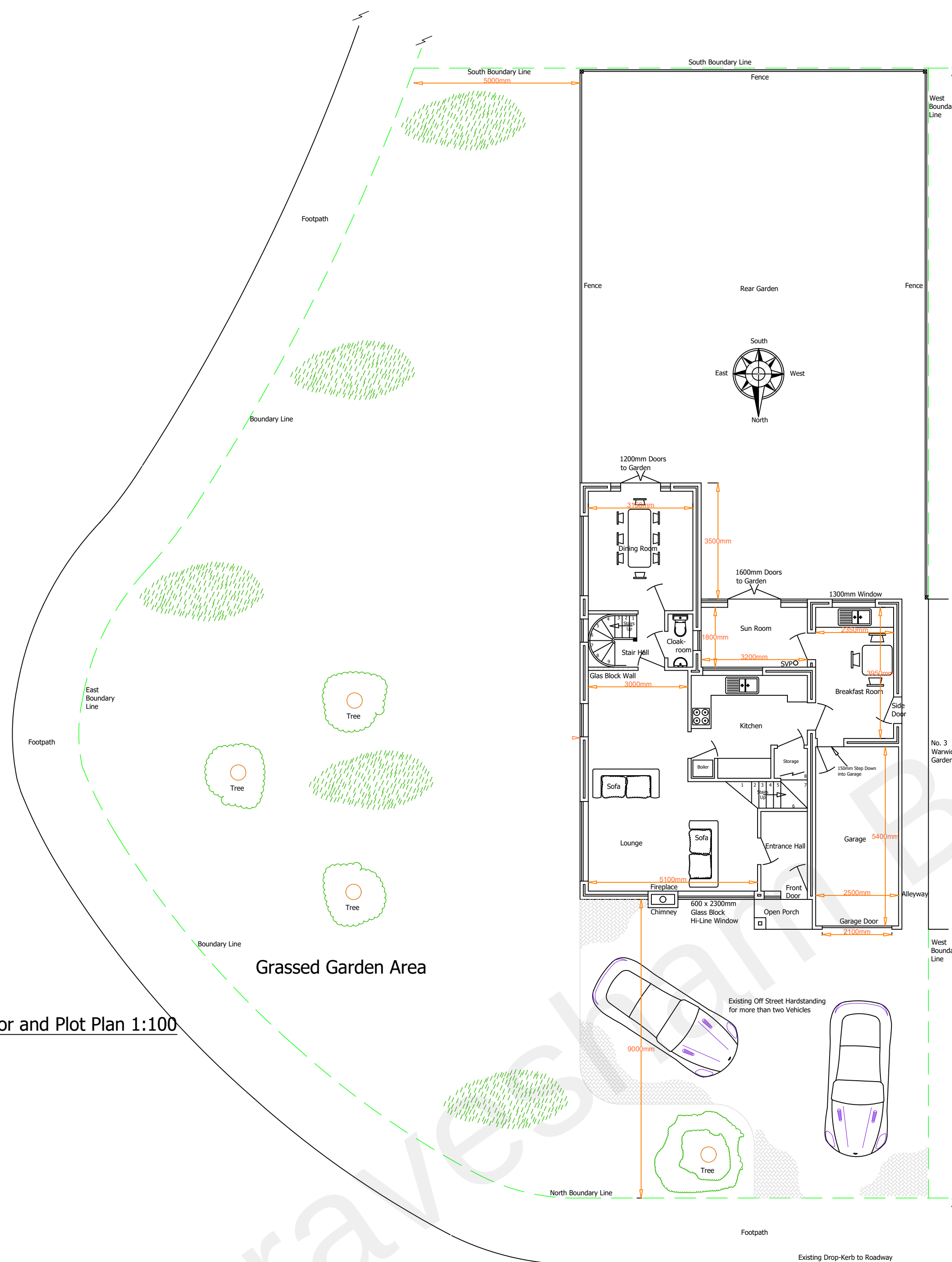
Proposed Fence Line Plot Plan 1:100
