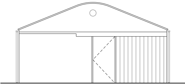
3 Existing East Elevation C-C
