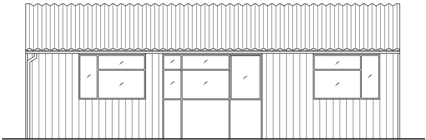
2 Existing North Elevation B-B
