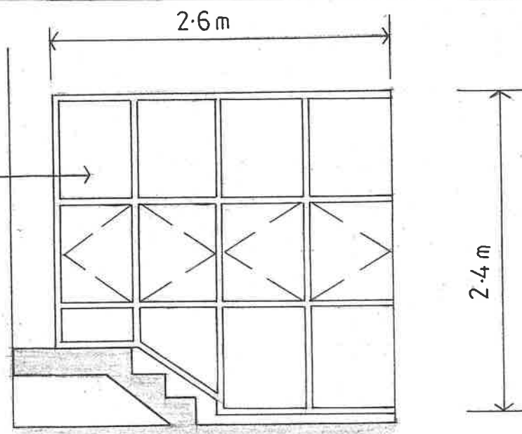
DETAIL A 1:20 ATA1 glazing unit in lightwell
