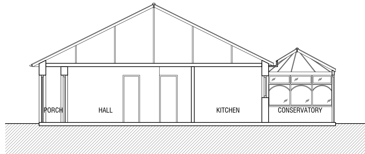
EXISTING SECTION Y-Y
