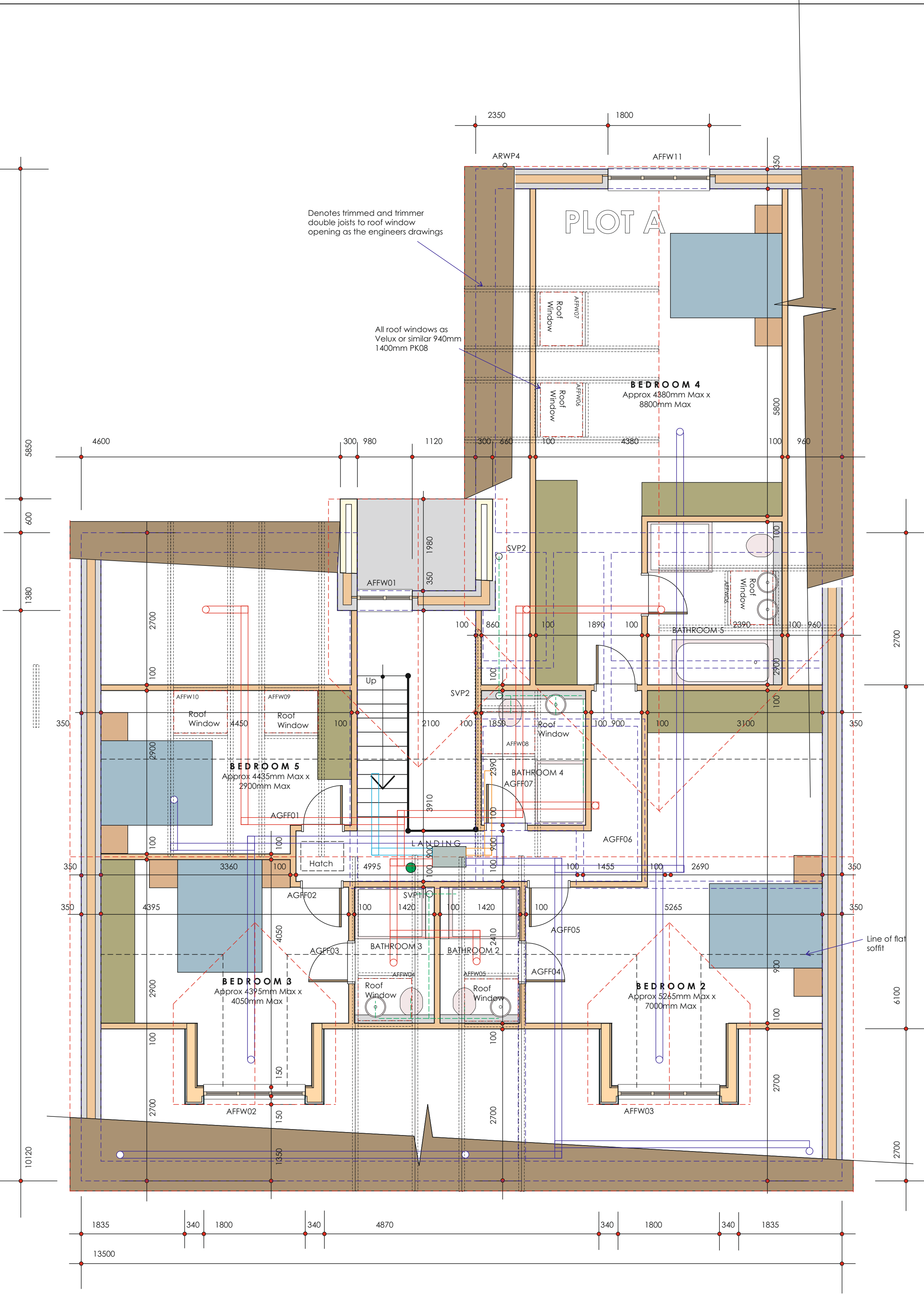
First Floor Plan-1:50
