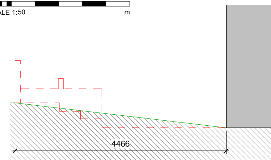
Indicative Proposed Section 1 : 50
