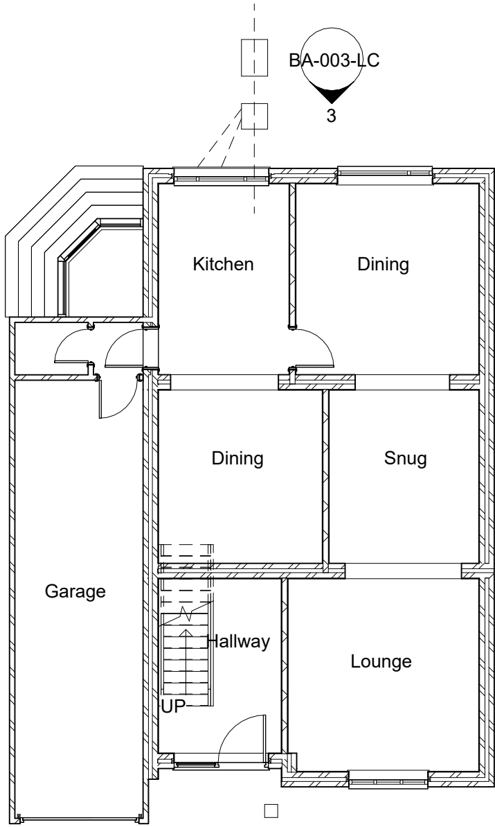
1 Ground Floor 1 : 100
