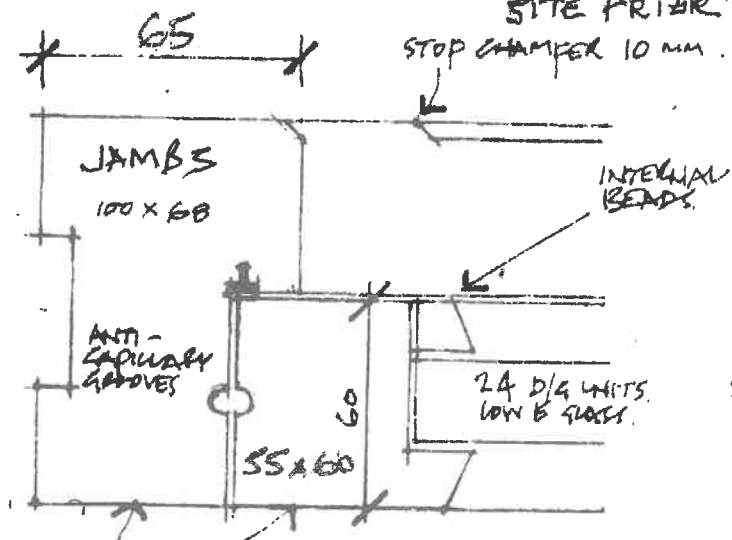
PLAN: WINDOW JAMBS
