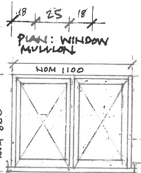
ELEV OF WINDOW
