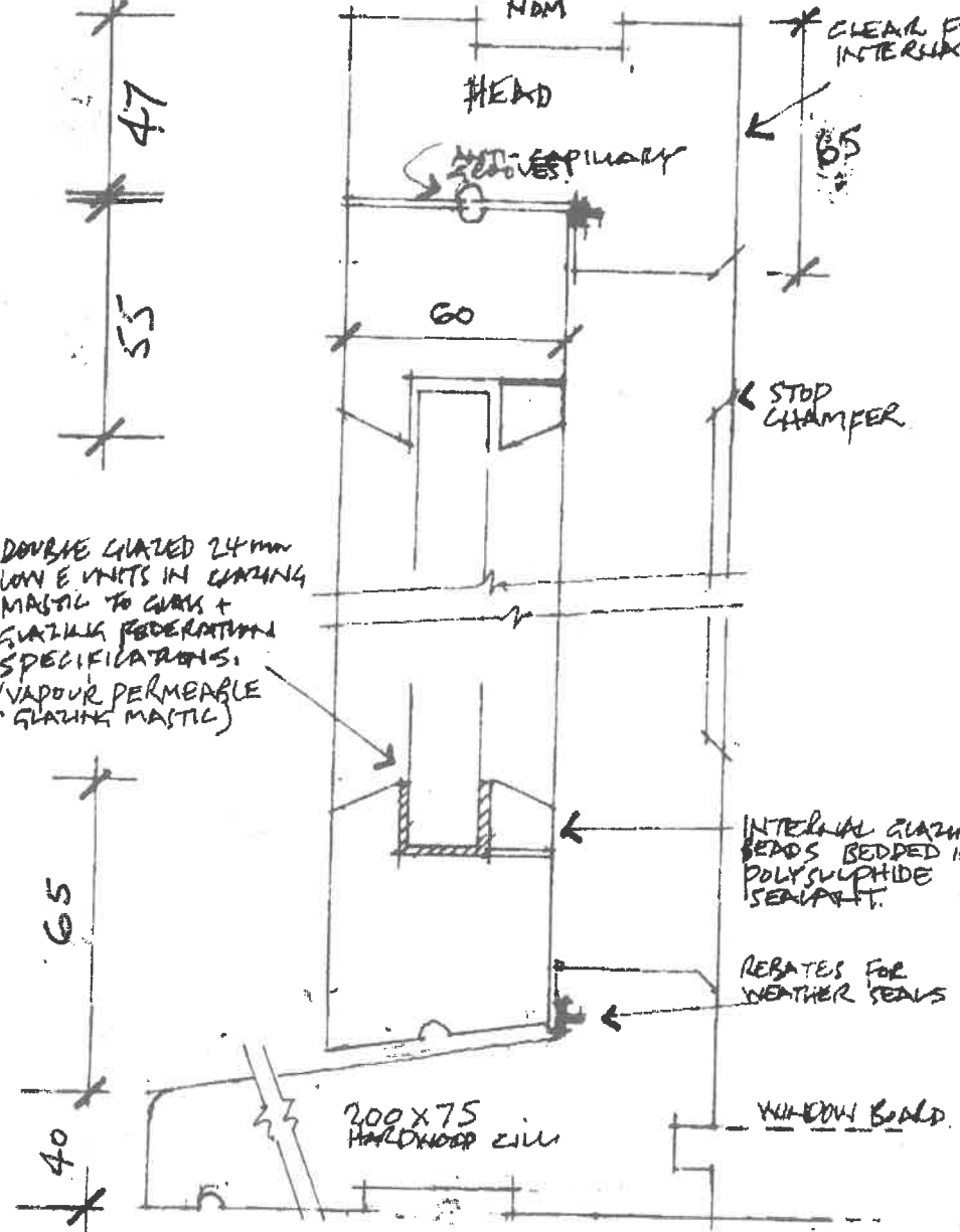
SECTION: WINDOWS
