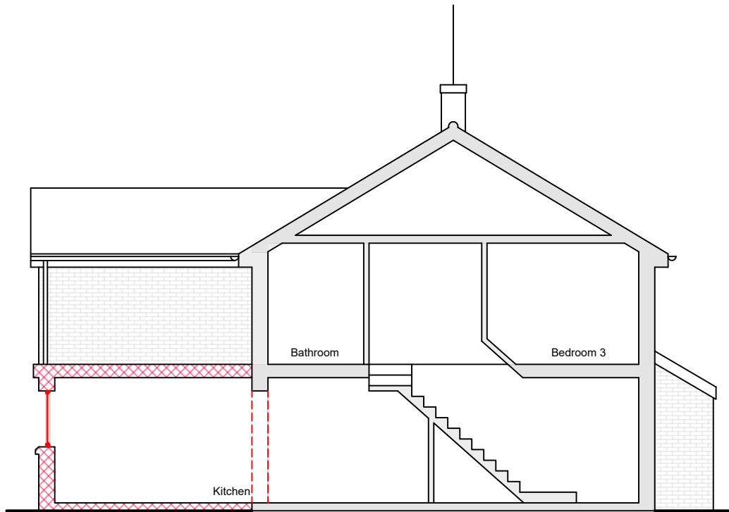
PROPOSED SIDE (North) ELEVATION / SECTION
