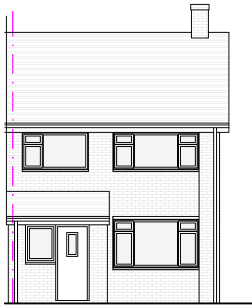
PROPOSED FRONT (West) ELEVATION
