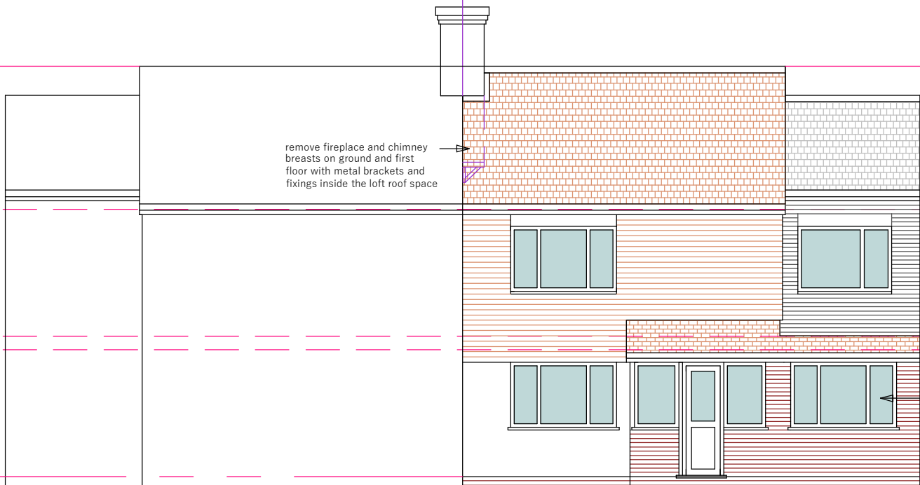
0 South Elevation
