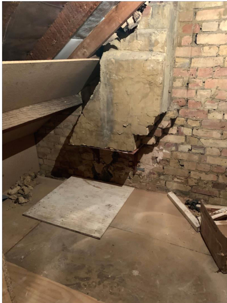
Chimney Support Brackets and Fixings
