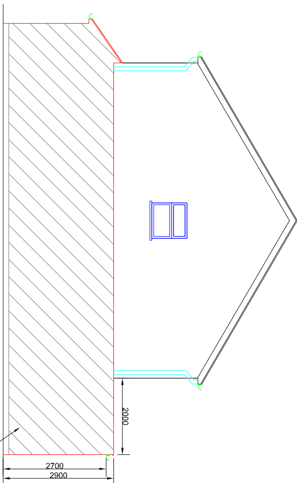
PROPOSED RIGHT SIDE VIEW
