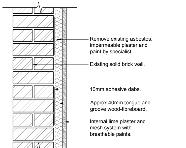
Proposed treatment to Wall Type 2
