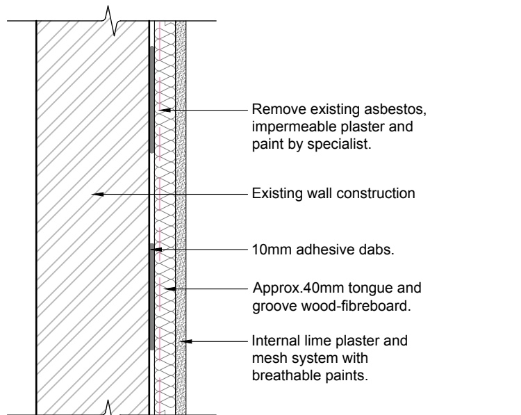
Proposed treatment to Wall Type 4
