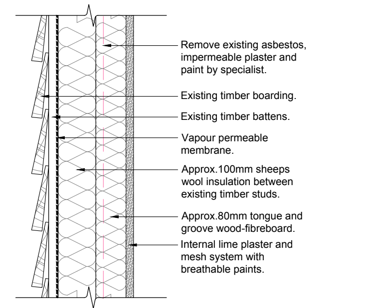
Proposed treatment to Wall Type 1
