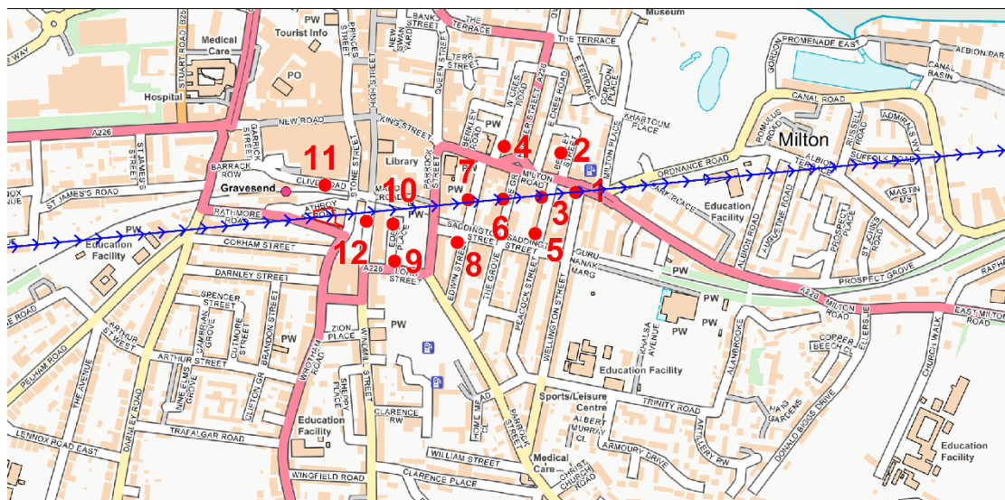
Figure 8 - Surveyed Locations. The blue arrows indicate the direction of the incoming DTT signals from Crystal Palace transmitter. The Site is delineated in red
