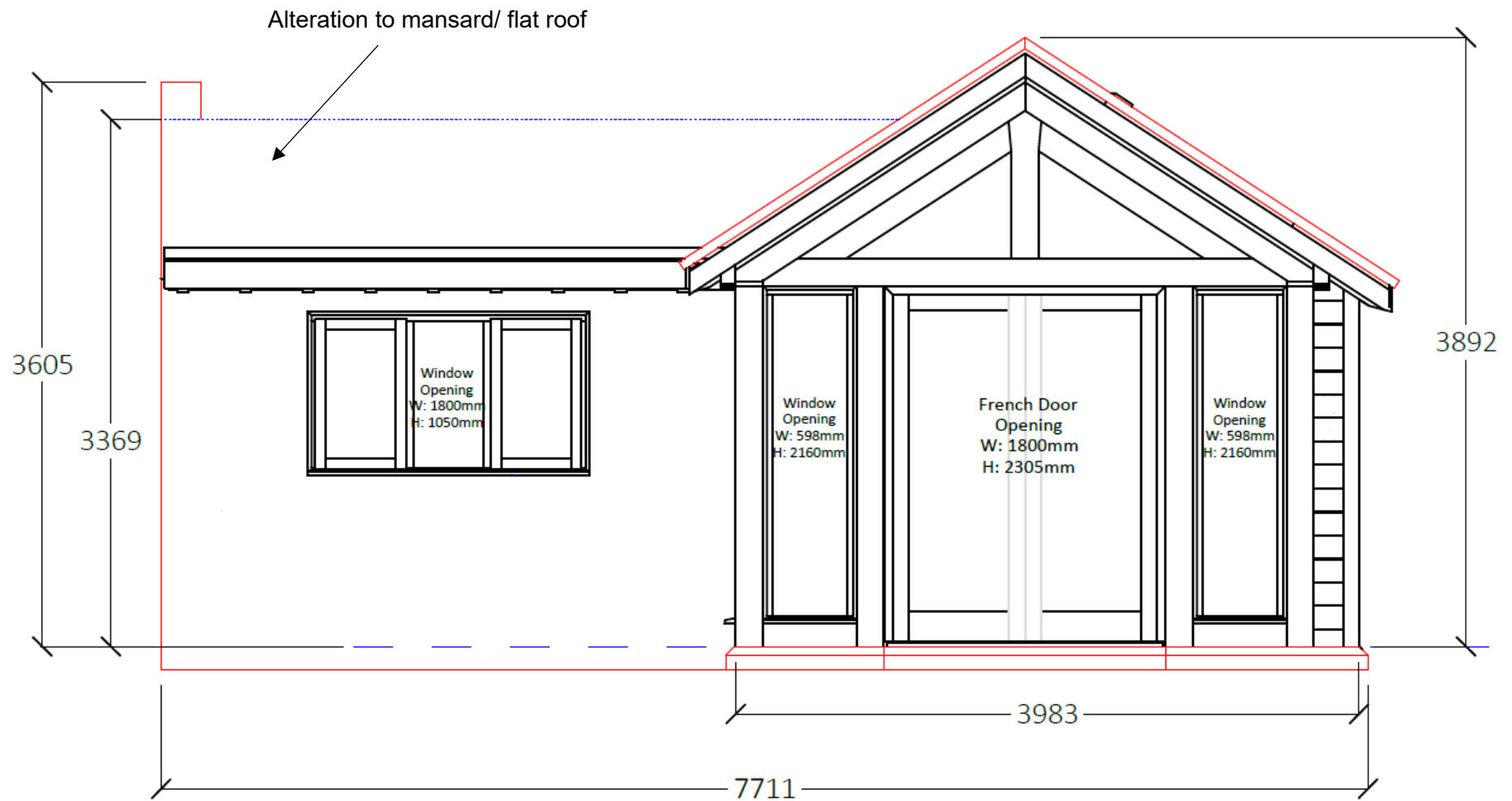
Rear Elevation
