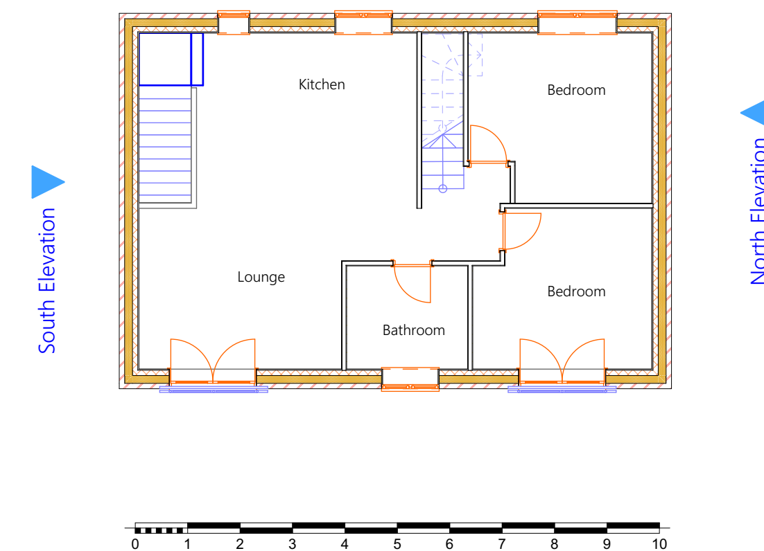
13 01 First Floor Proposed 1:100
