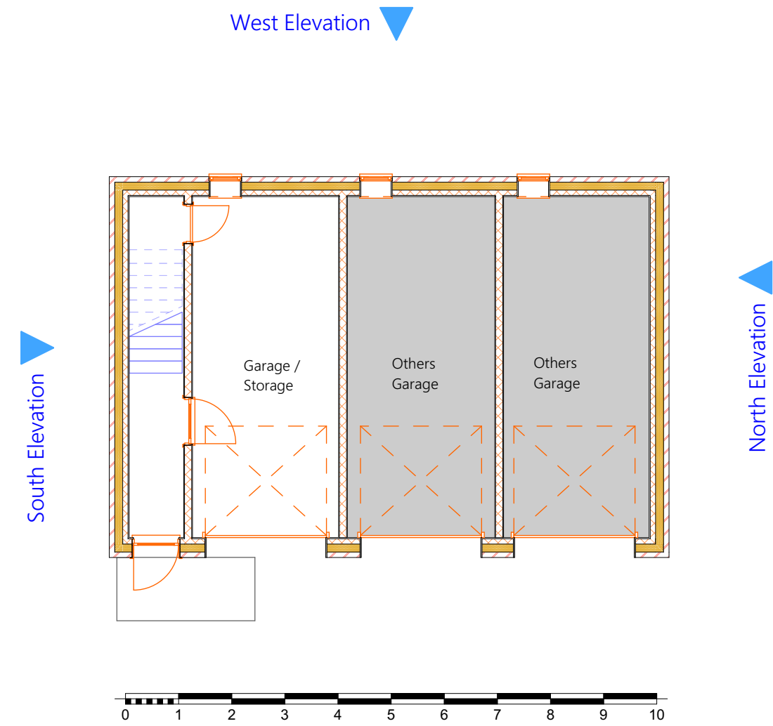
5 GF Ground Floor Existing 1:100
