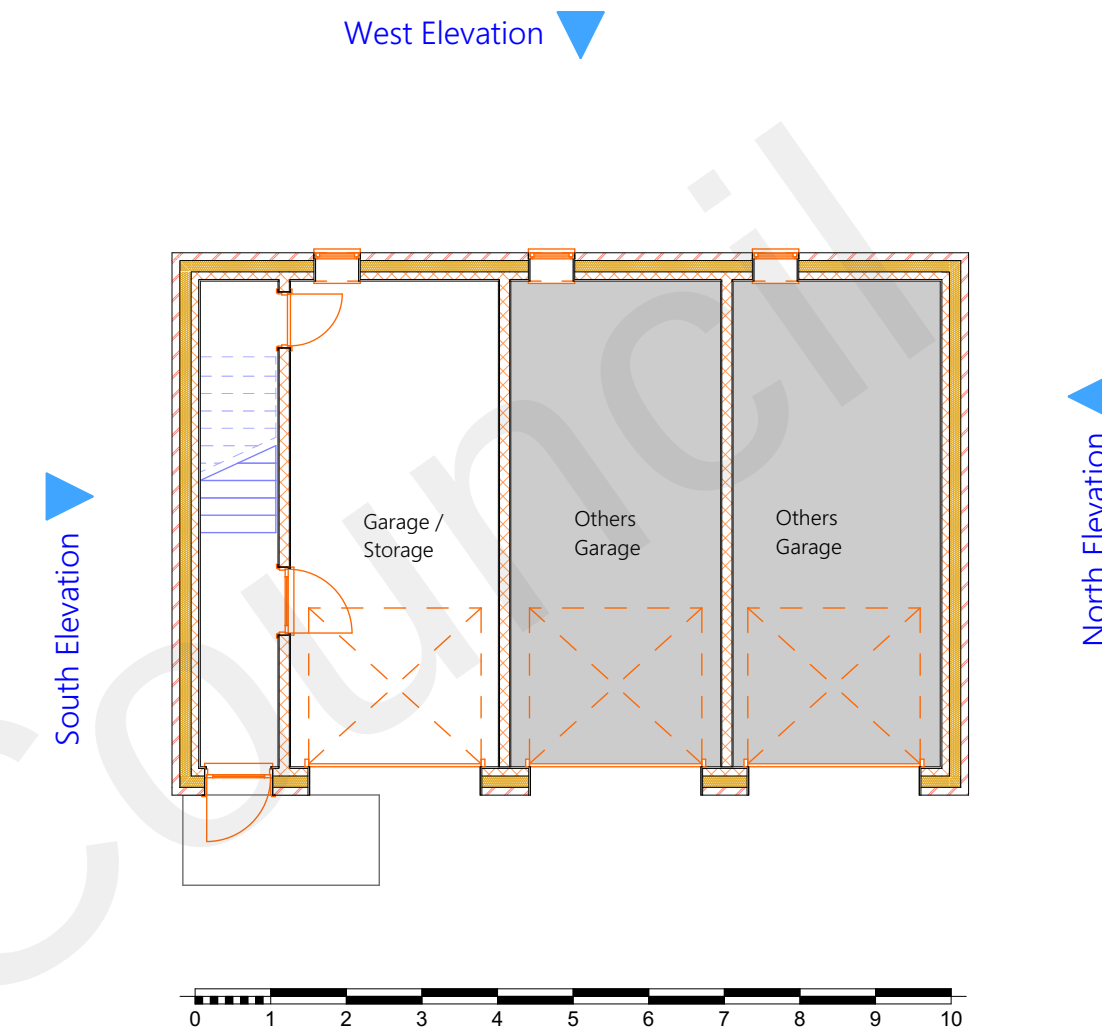
12 GF Ground Floor Proposed 1:100
