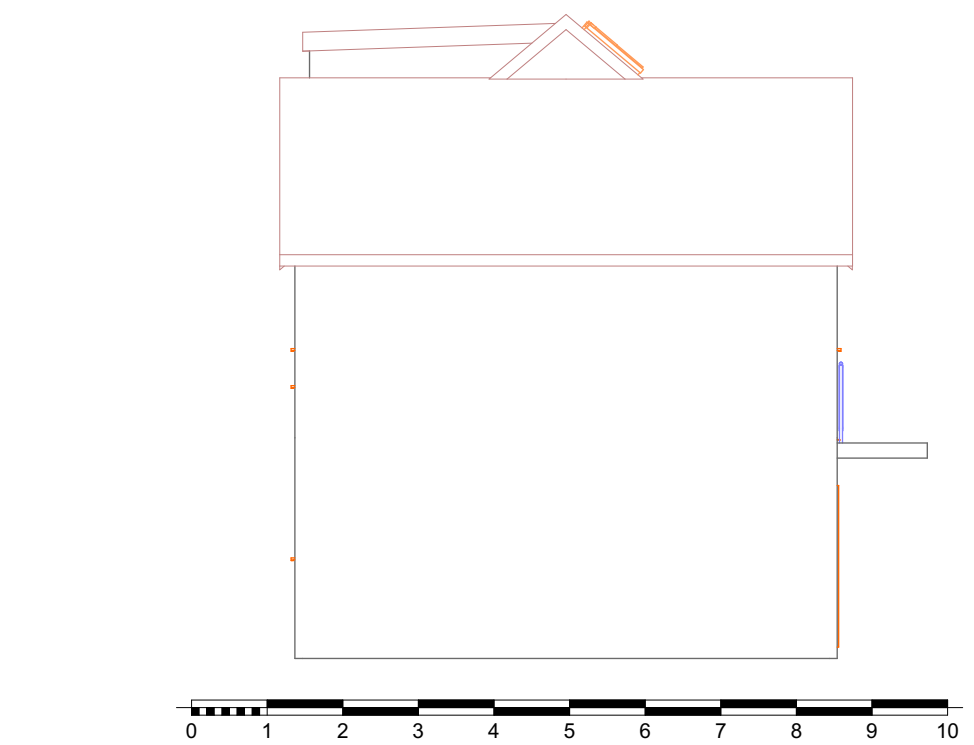
11 South Elevation Proposed 1:100
