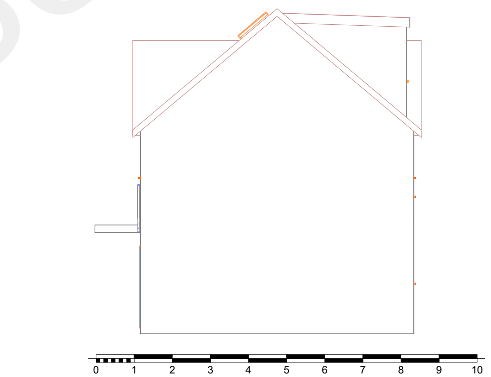
10 North Elevation Proposed 1:100
