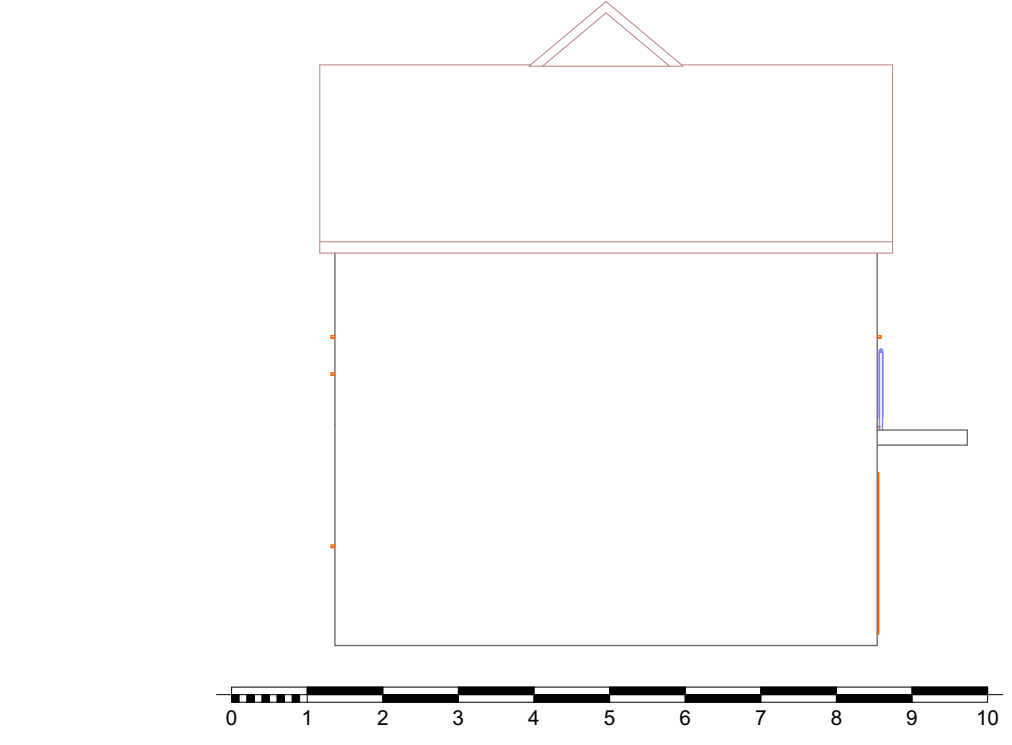
4 South Elevation Existing 1:100
