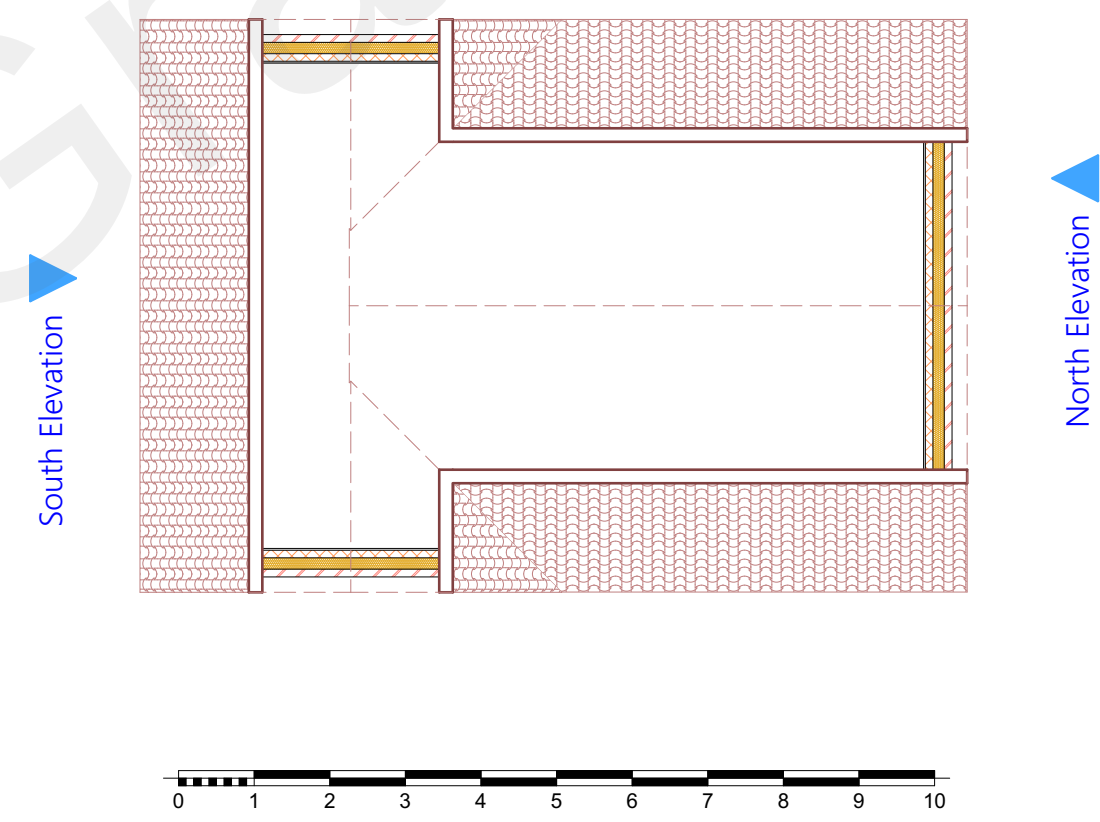
7 Roof -Existing 1:100
