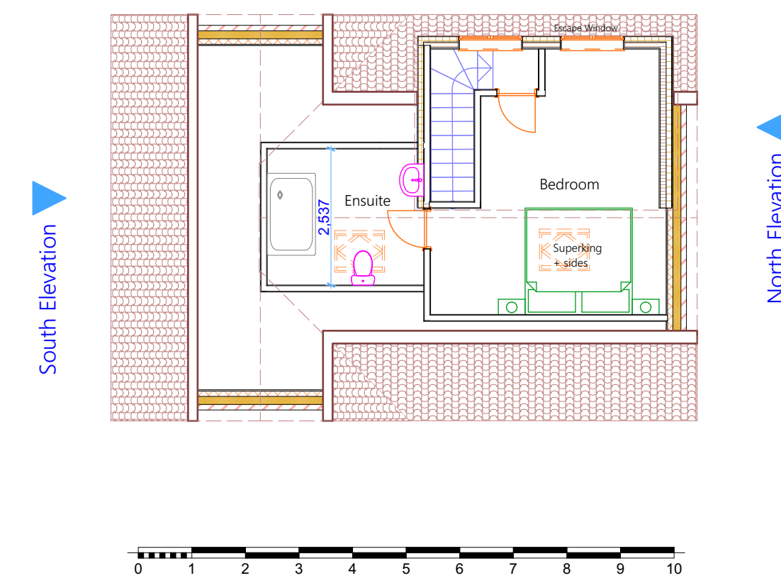
14 Roof Proposed 1:100
