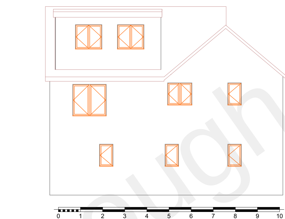
9 West Elevation Proposed 1:100
