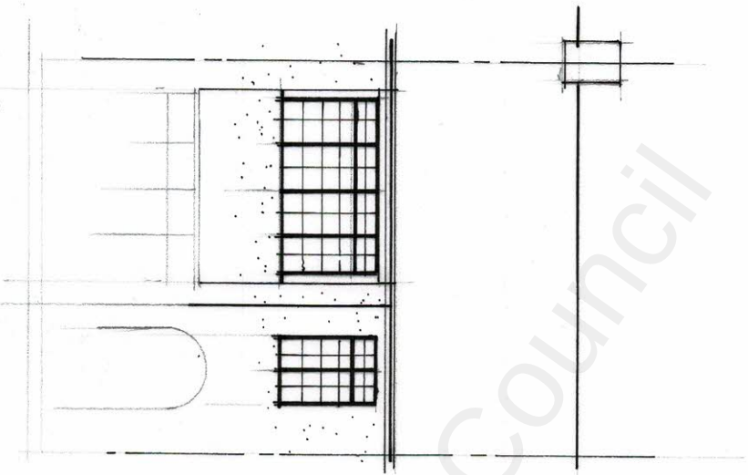
EXISTING FRONT ELEVATION (WITHOUT VELUX WINDOWS)
