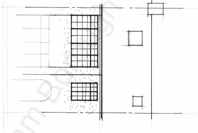
PROPOSED FRONT ELEVATION (WITH 2 VELUX WINDOWS)
