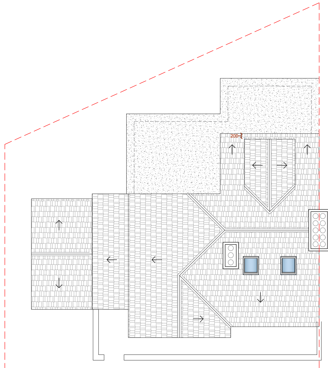
ROOF PLAN
