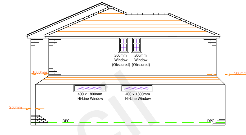
Proposed Side (North) Elevation 1:100
