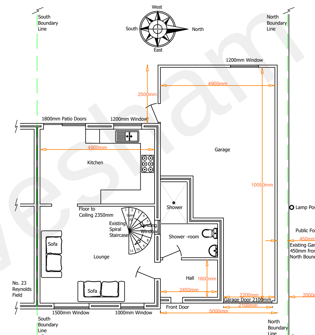
Existing Ground Floor Plan 1:100
