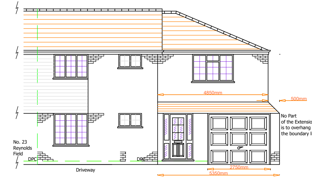
Proposed Front (East) Elevation 1:100
