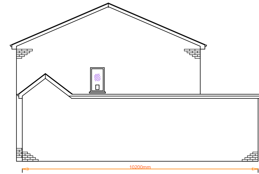
Existing Side (North) Elevation 1:100
