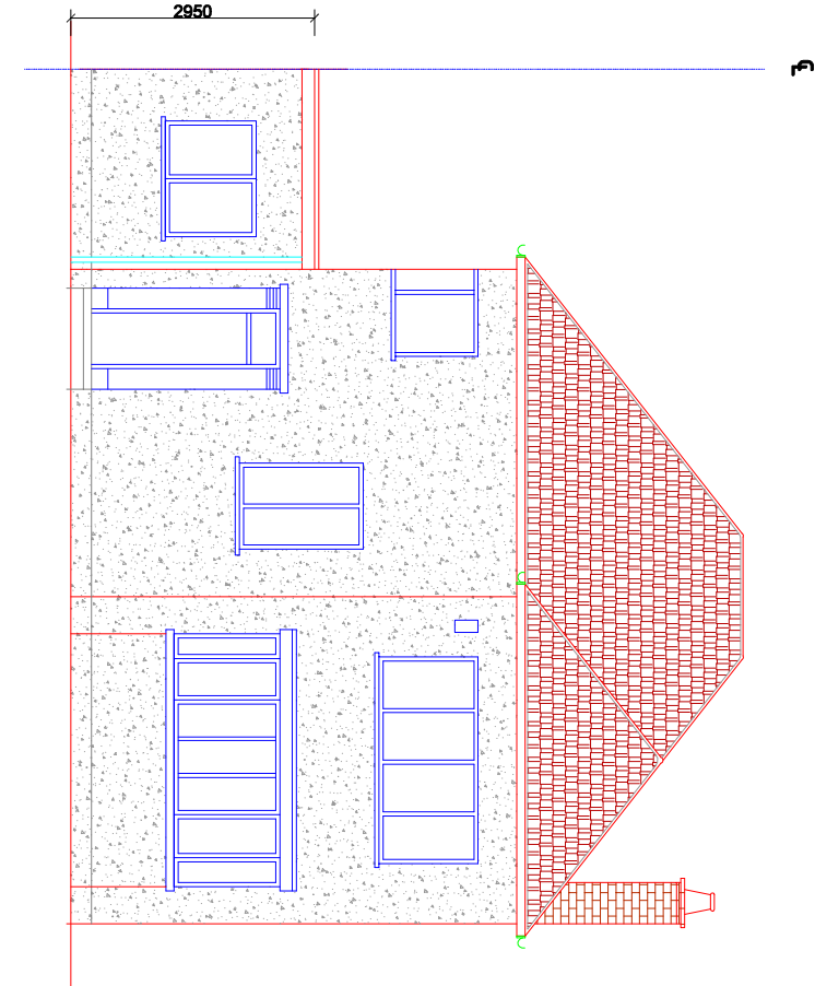
EXISTING FRONT VIEW
