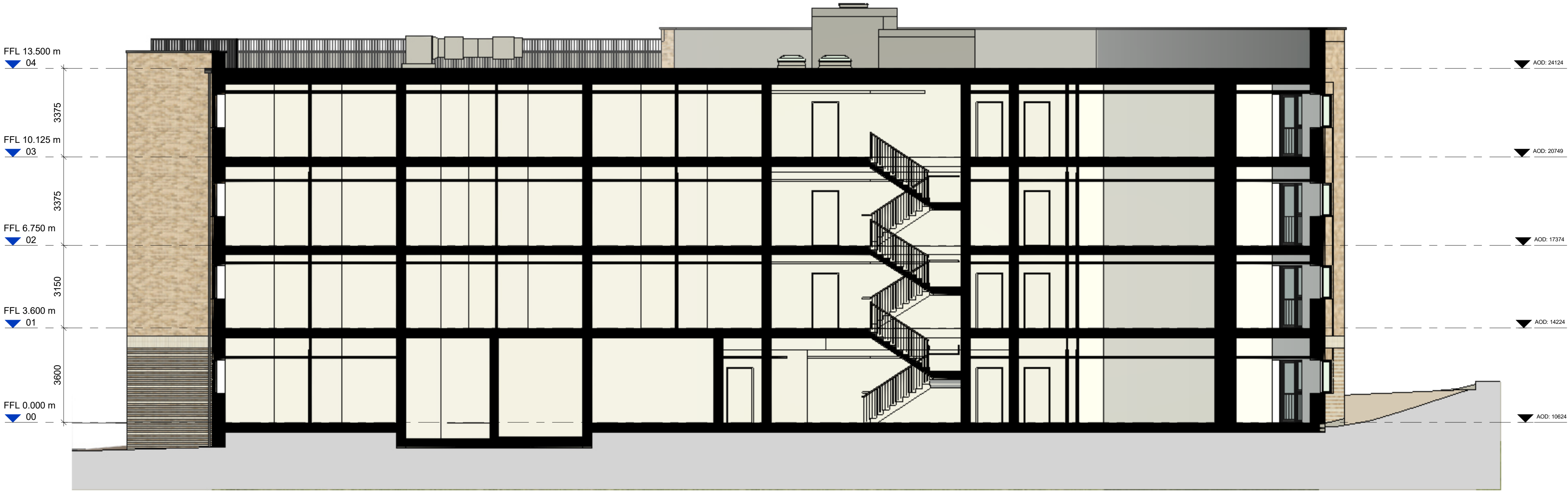
Apartment Section 2 1 : 100
