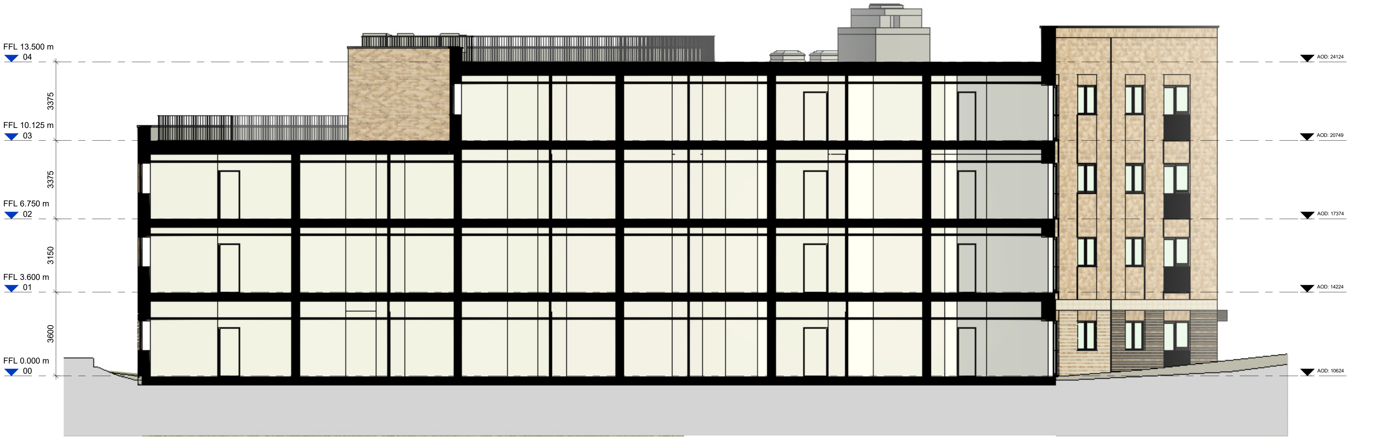
Apartment Section 1 1 : 100
