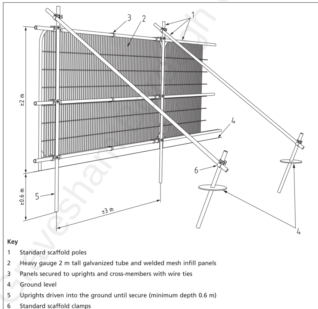
Figure 10 Default specifications for Tree Protection Fencing
