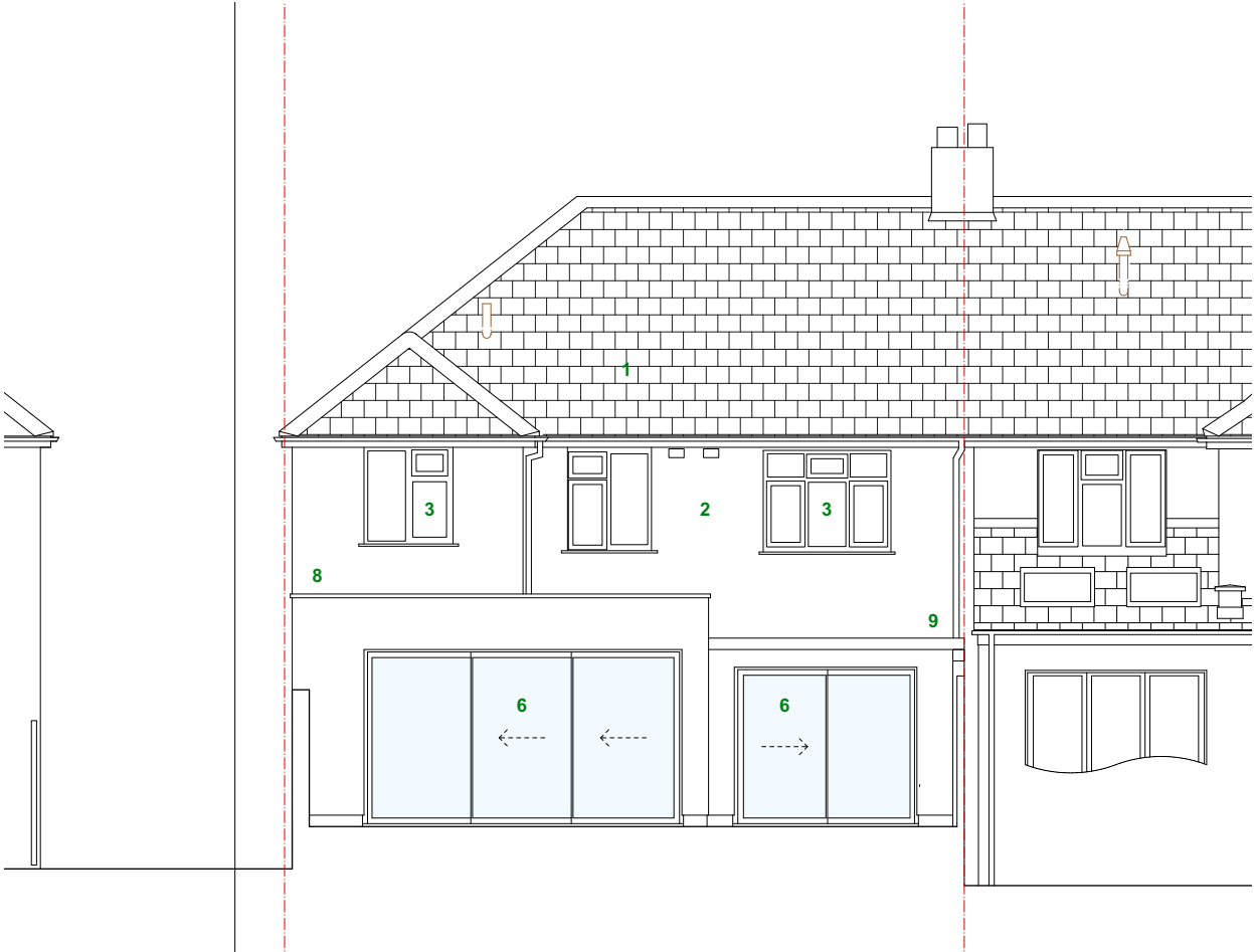
02 | Rear (East) Elevation Proposed
