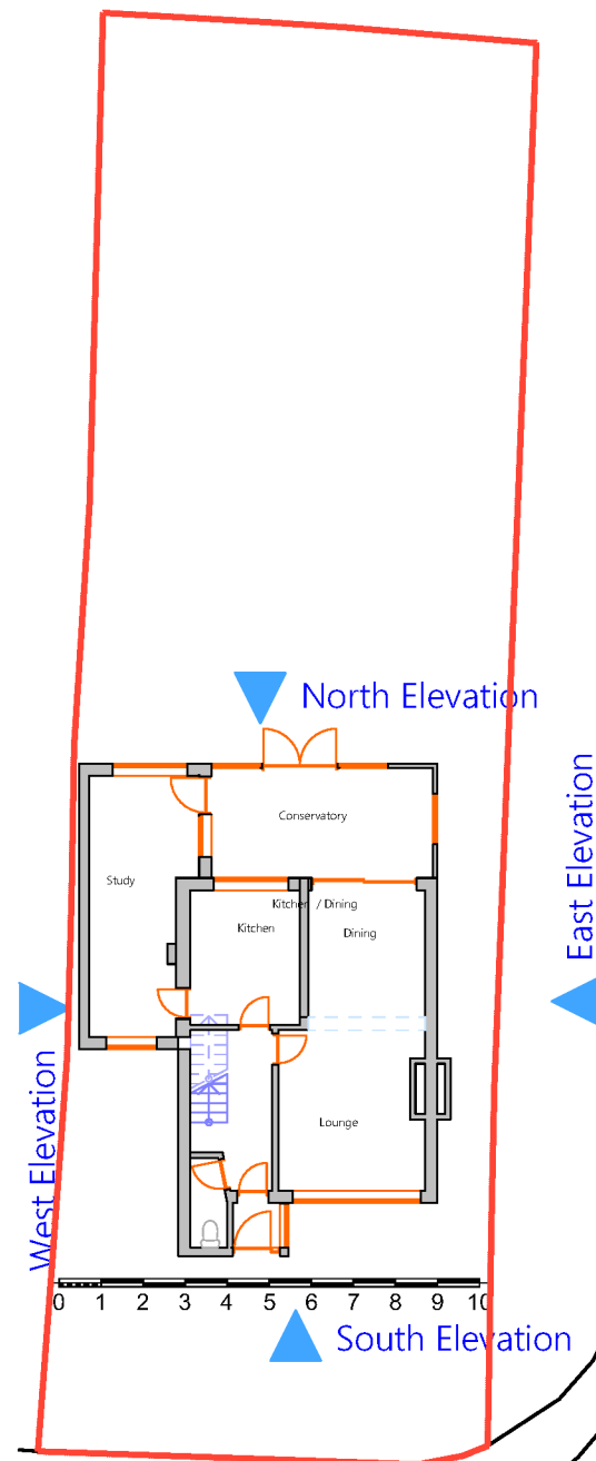
2 Site Plan Existing 1:200
