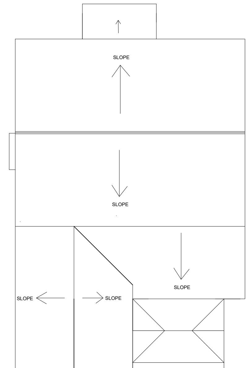
ROOF PLAN EXISTING
