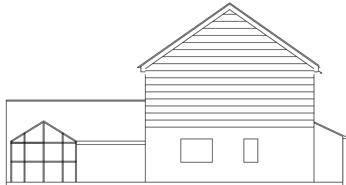
EXIST. SOUTH ELEVATION
