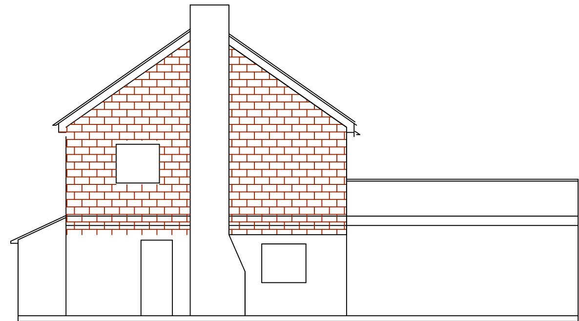
EXIST. NORTH ELEVATION
