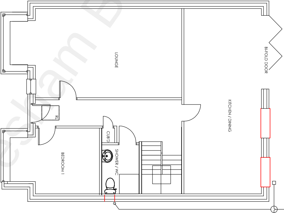
ground floor plan Plot 2
