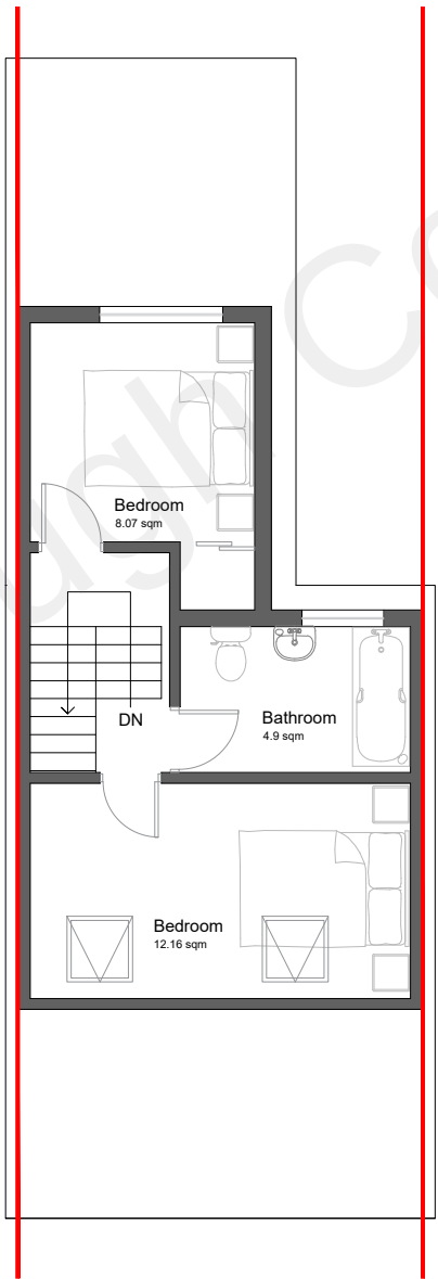
Proposed Loft Floor Plan
