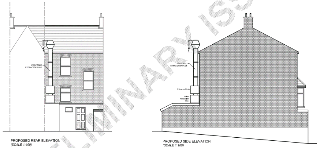
Figure 2: Proposed rear elevation showing ductwork
