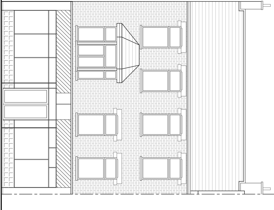
EXISTING FRONT ELEVATION (NO CHANGES PROPOSED) (SCALE 1:100)
