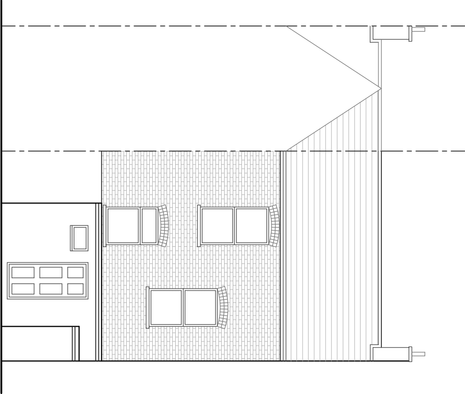
EXISTING FRONT ELEVATION (NO CHANGES PROPOSED) (SCALE 1:100)
