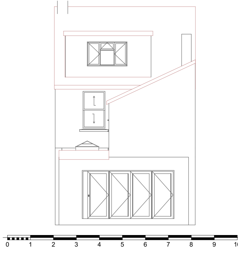
8 South Elevation Proposed 1:100
