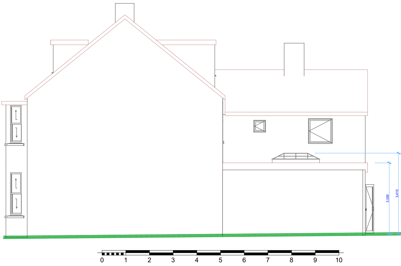
6 West Elevation Proposed 1:100
